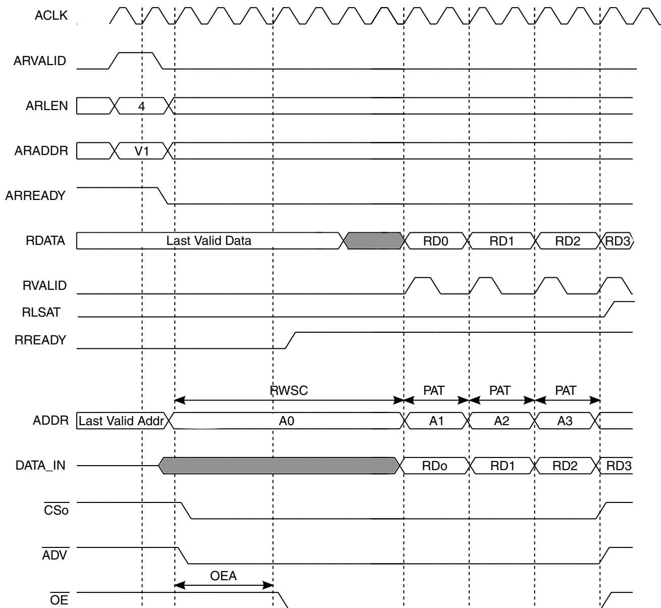
Figure 9-68. PAT = 2
