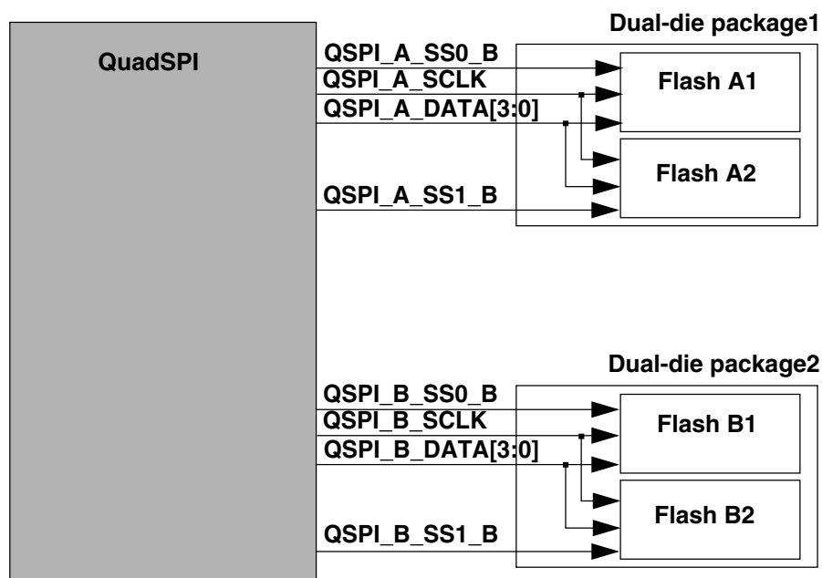
Figure 10-23. Dual-die support
