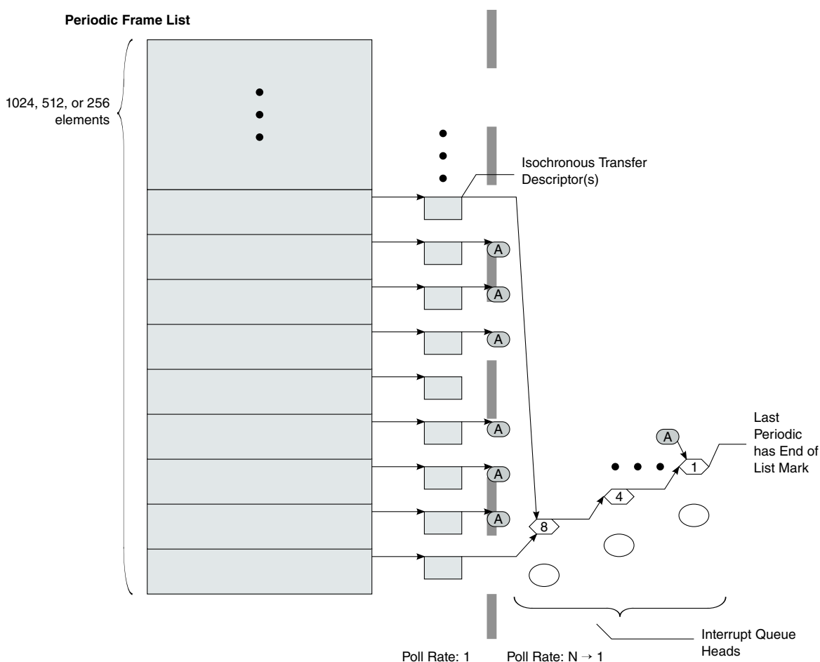
Figure 11-70. Example Periodic Schedule
