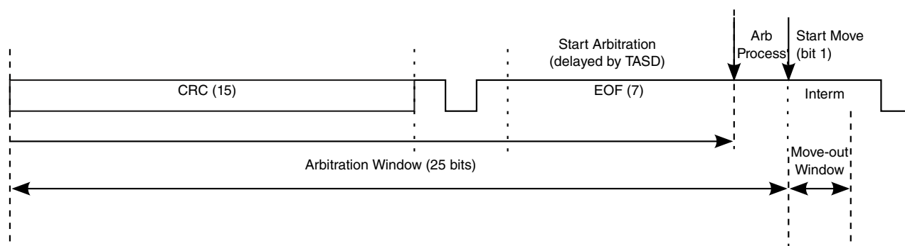
Figure 15-4. Arbitration and Move-Out Time Windows
