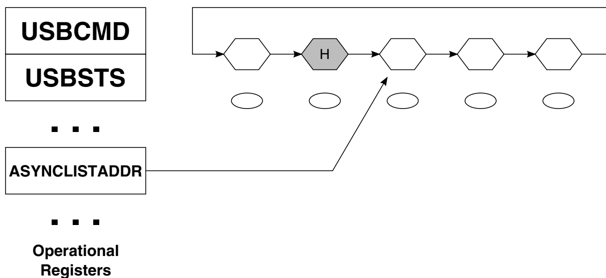
Figure 11-66. General Format of Asynchronous Schedule List
