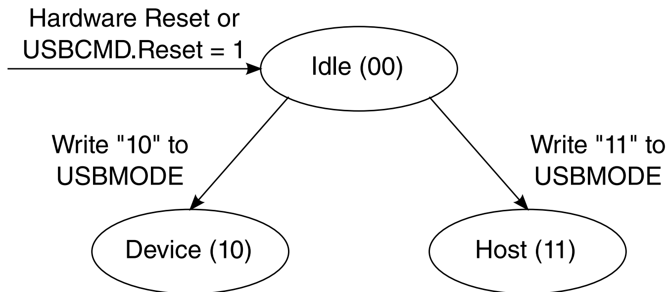
Figure 11-60. Controller Mode
