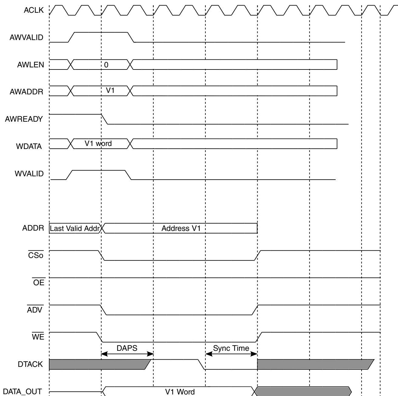
Figure 9-72. DAPS = 2
