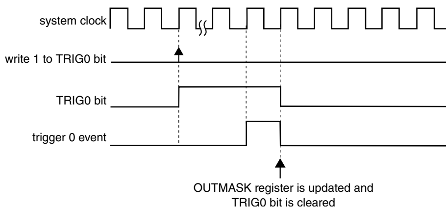
Figure 12-58. OUTMASK synchronization with (SYNCMODE = 0), (HWTRIGMODE = 0), (SYNCHOM = 1), (PWMSYNC = 0), and a hardware trigger was used
