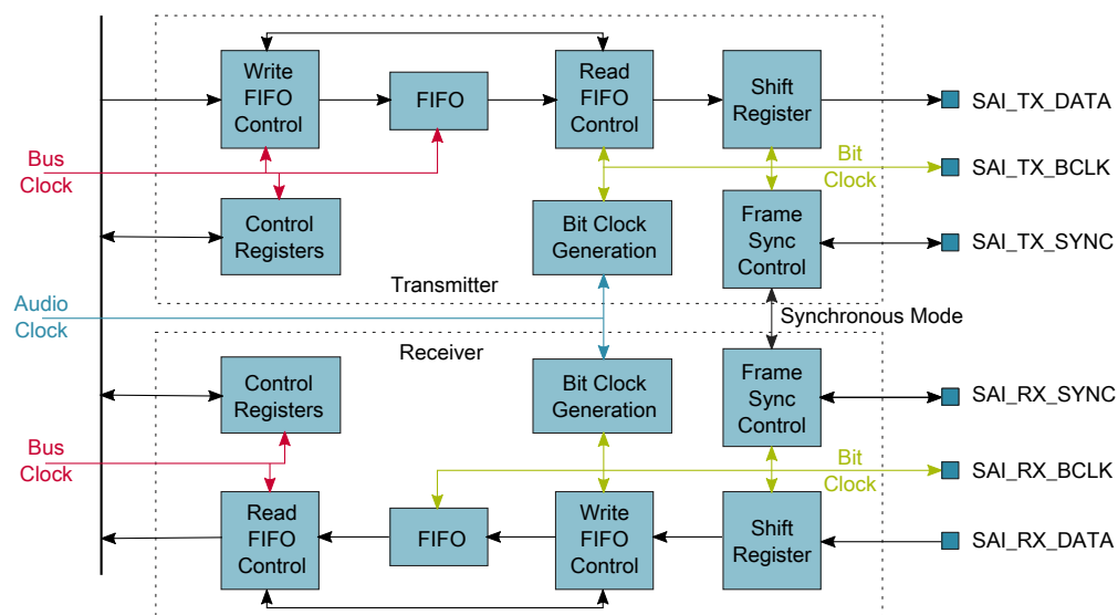
Figure 13-117. I²S/SAI block diagram
