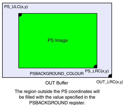
Figure 13-106. OUT Buffer
