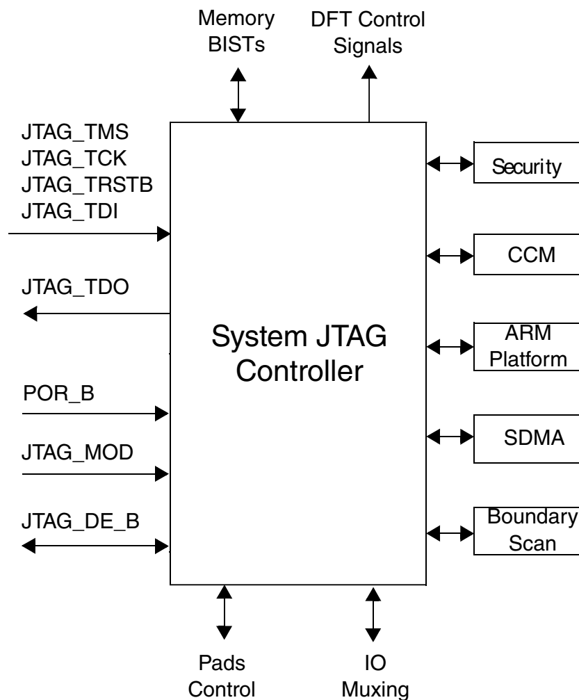
Figure 4-26. SJC Connections
