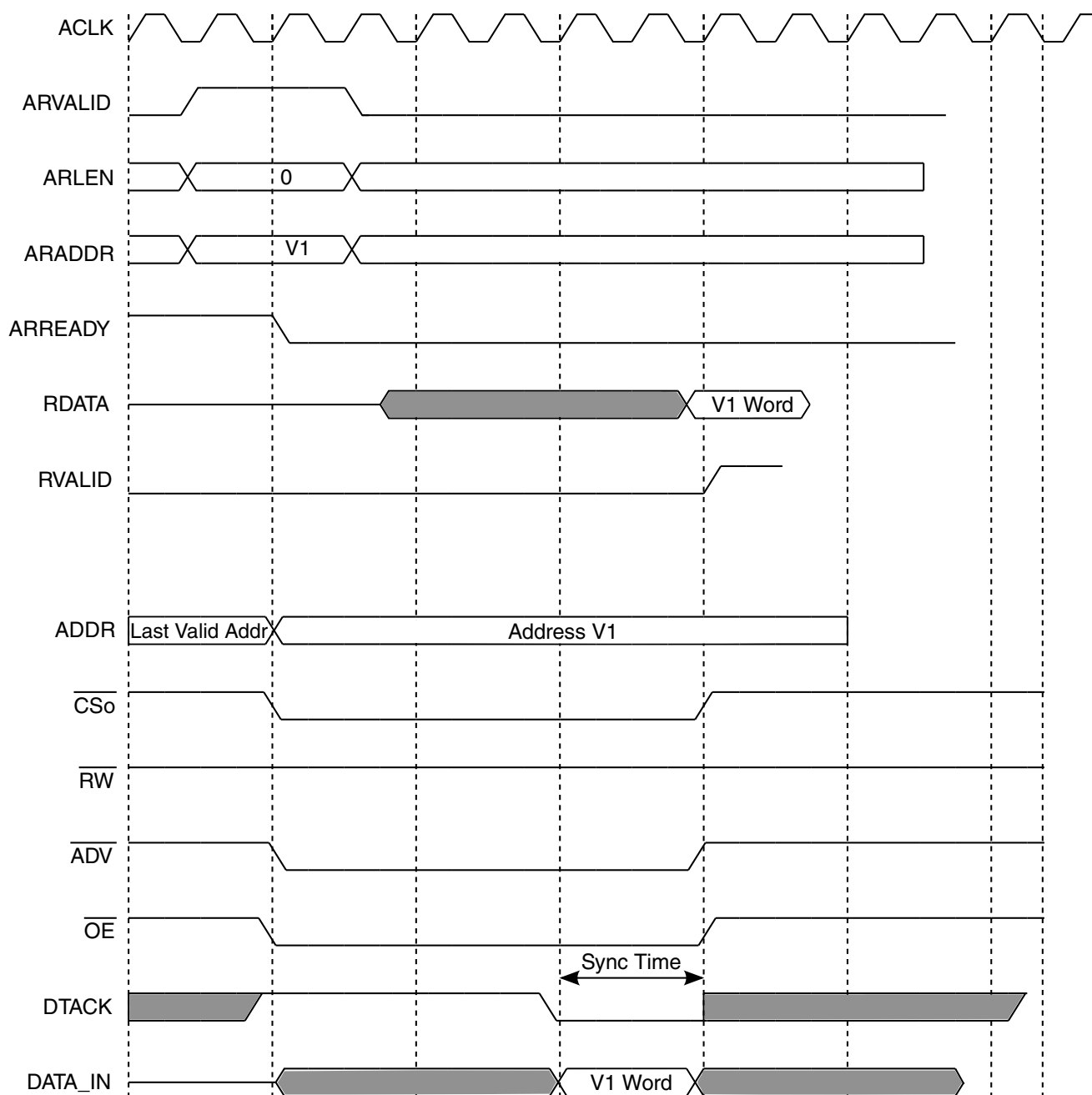
Figure 9-70. DAPS = 0
