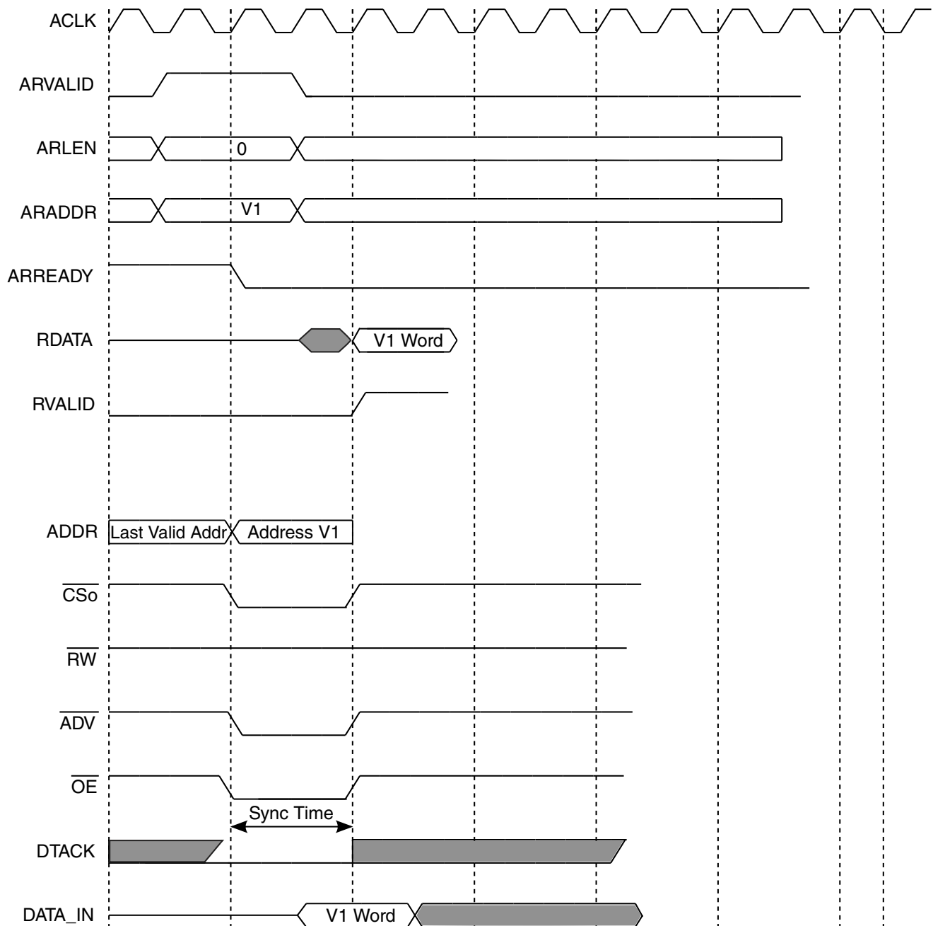
Figure 9-71. DAPS = 0
