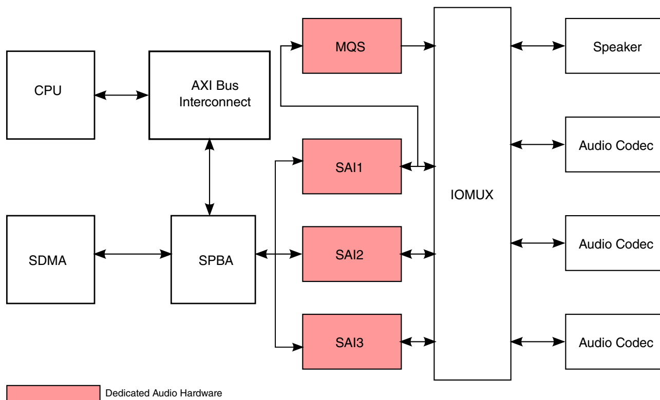
Figure 13-2. Audio subsystem block diagram
