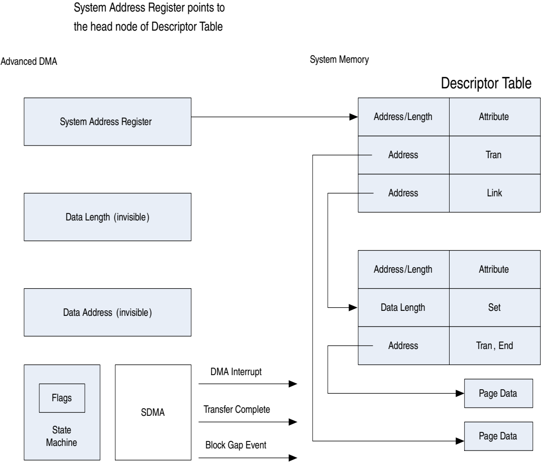
Figure 10-43. Concept and Access Method of ADMA1 Descriptor Table
