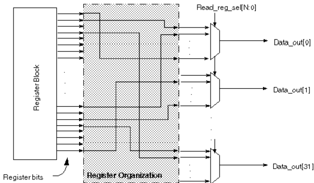
Figure 11-34. SIM Read Registers
