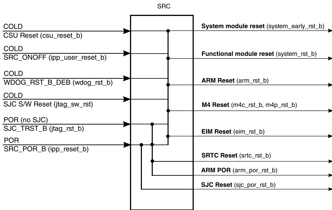
Figure 6-9. SRC inputs and outputs
