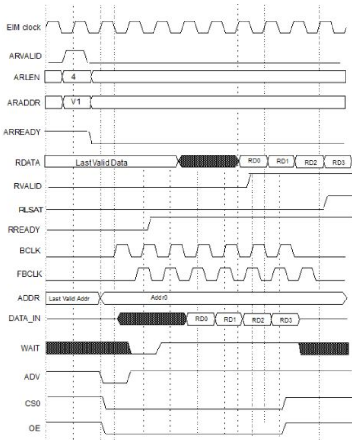
Figure 9-66. SRD=1,BCD=0,BCS=0,RWSC=1,RADVA=0,RADVN=0,RFL=0,RL=0
