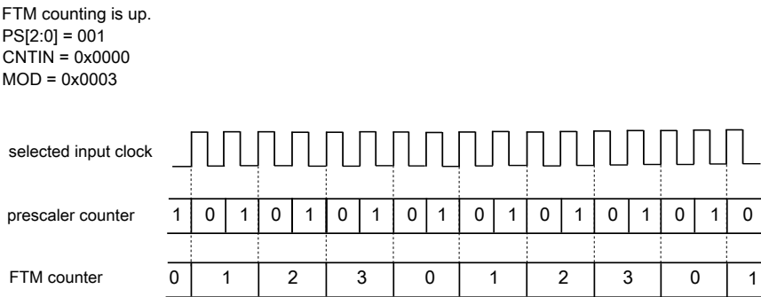
Figure 12-7. Example of the prescaler counter
