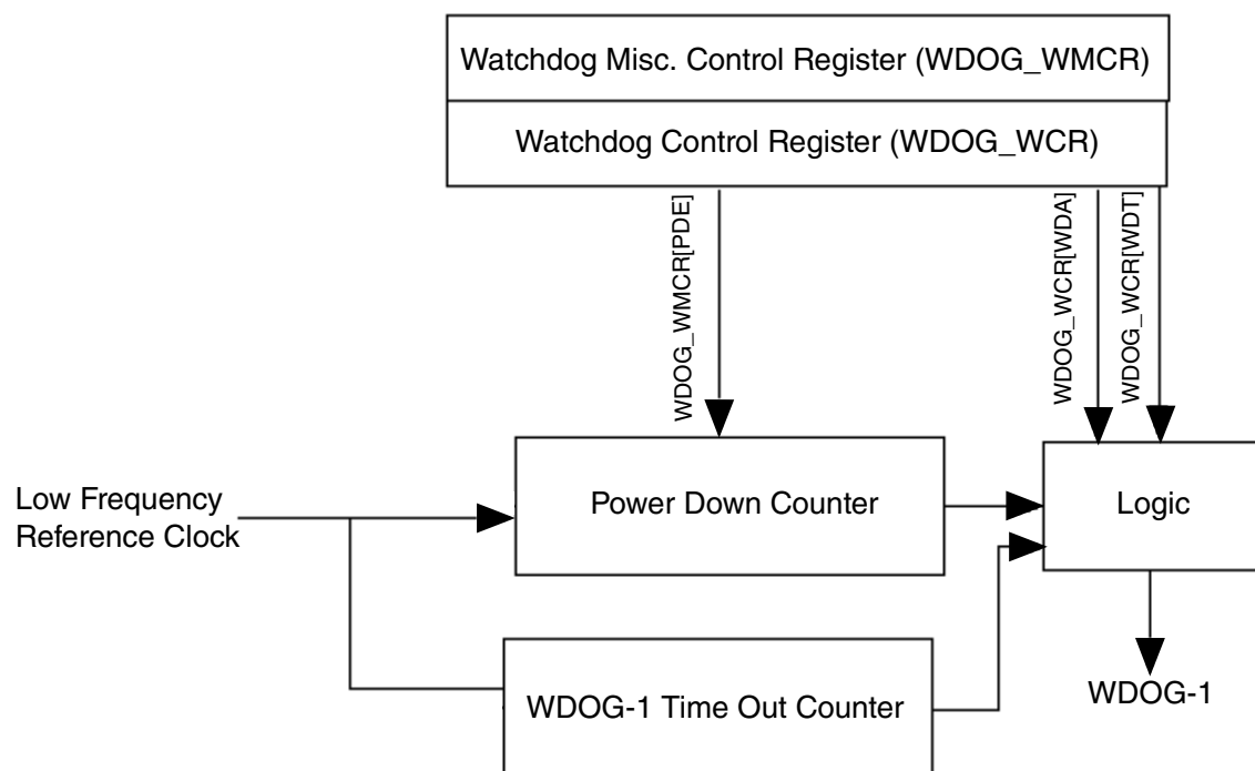
Figure 6-15. WDOG_B generation
