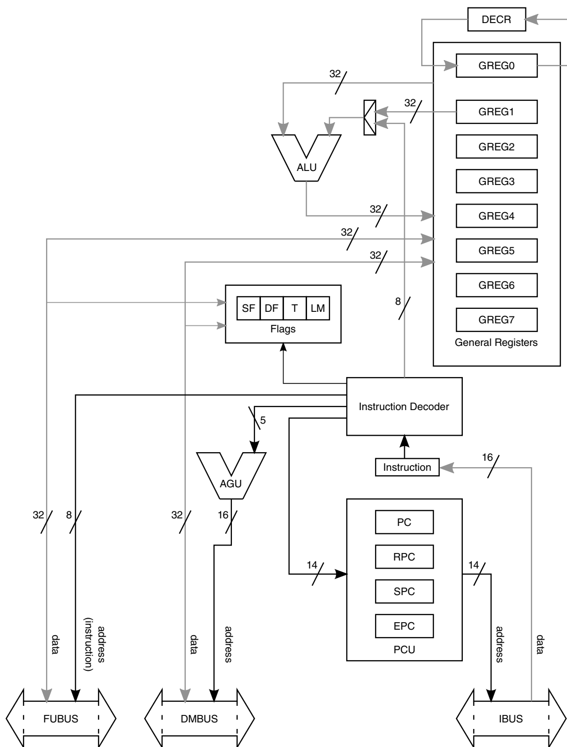
Figure 7-1. SDMA Core
