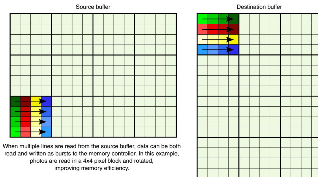
Figure 13-98. Rotated Sub-blocks
