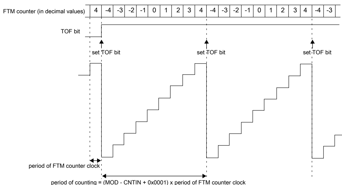
Figure 12-8. Example of FTM up and signed counting
