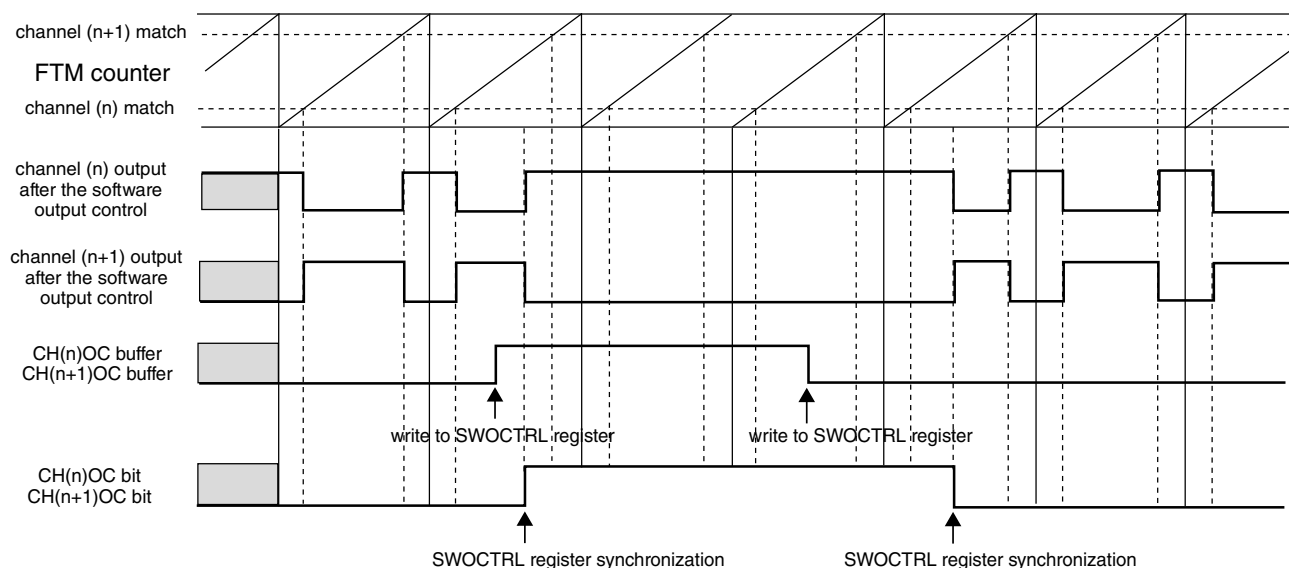
Figure 12-69. Example of software output control in Combine and Complementary mode
