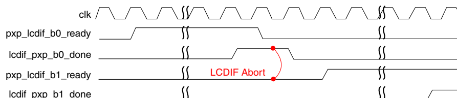
Figure 13-104. LCDIF Abort
