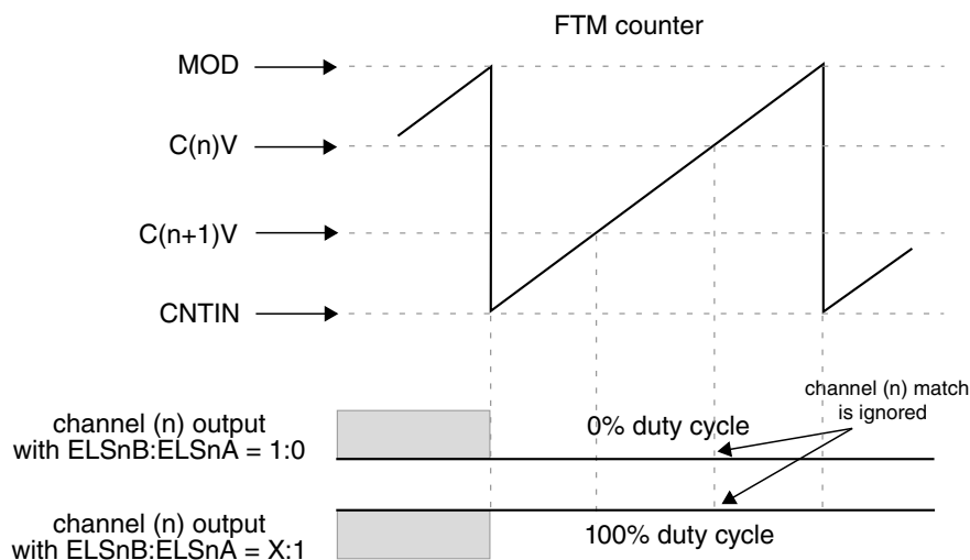
Figure 12-39. Channel (n) output if (\text{CNTIN} < C(n)V < \text{MOD}) and (\text{CNTIN} < C(n+1)V < \text{MOD}) and (C(n)V > C(n+1)V)
