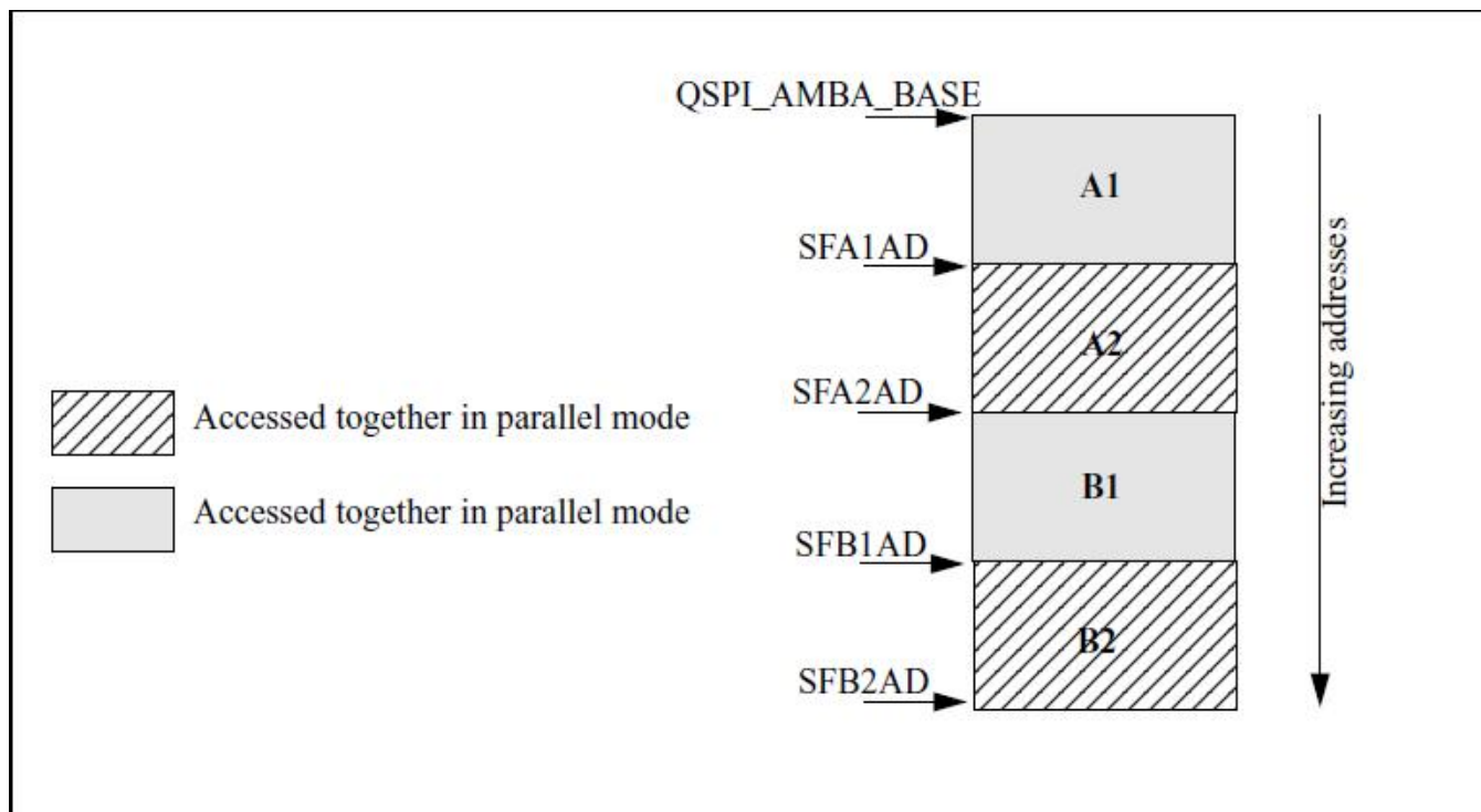
Figure 10-21. Flash addressing
