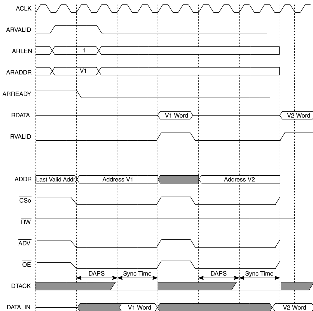
Figure 9-73. DAPS = 2 CSREC = 2
