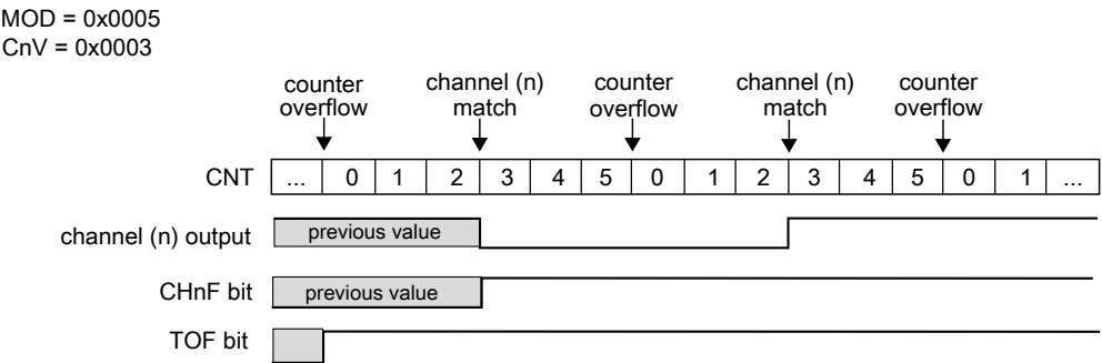
Figure 12-20. Example of the Output Compare mode when the match toggles the channel output
