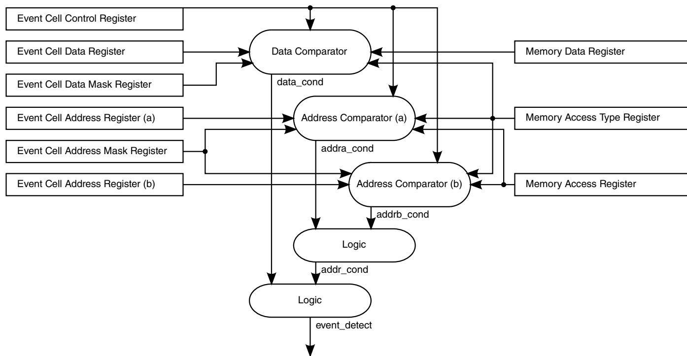
Figure 7-12. Event Cell Architecture
