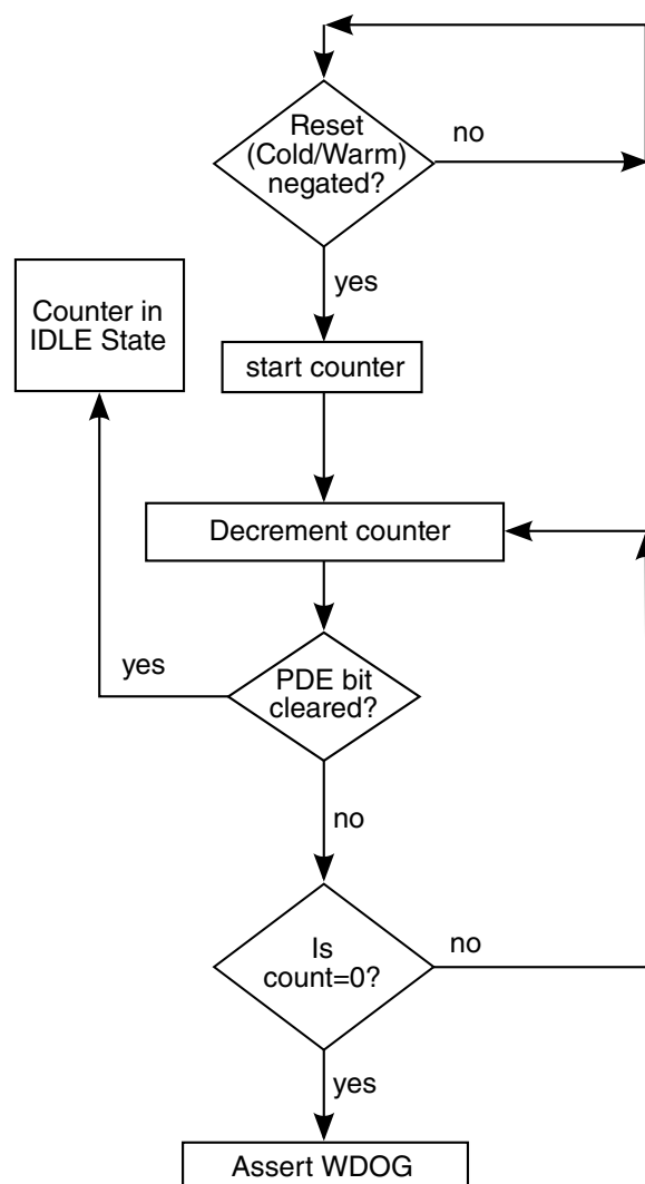
Figure 6-18. Power-Down Counter Flow Diagram
