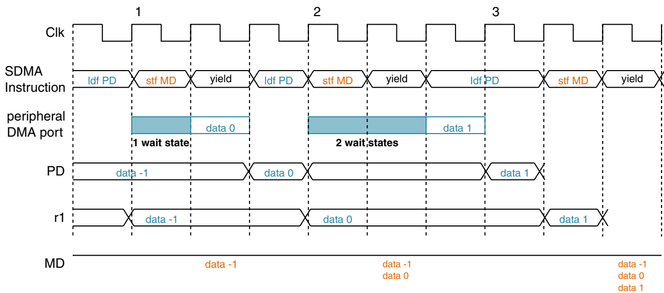
Figure 7-19. Peripheral to External Memory Example (1)
