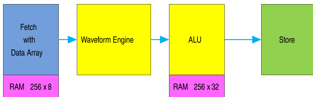
Figure 13-113. Block Diagram
