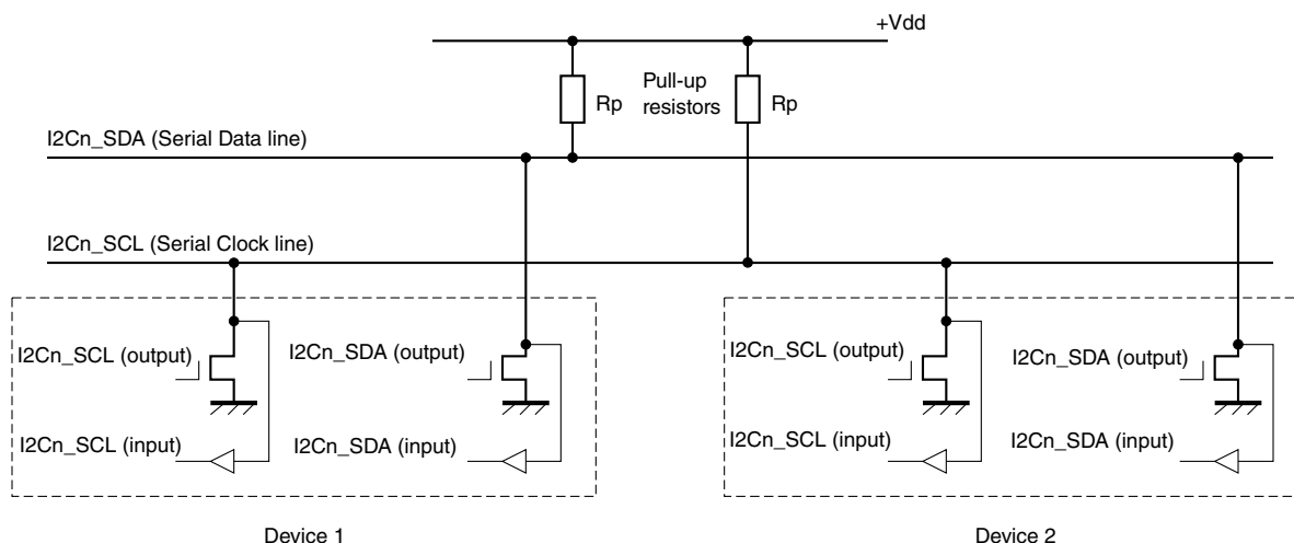
Figure 15-6. Connection of devices to I2C bus
