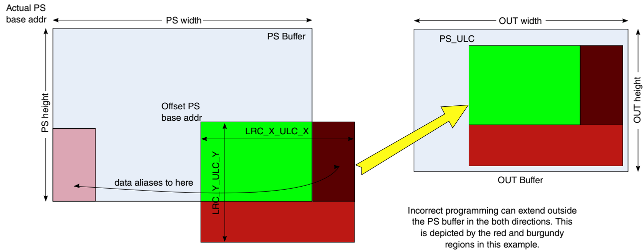
Figure 13-108. Example with Invalid Parameters
