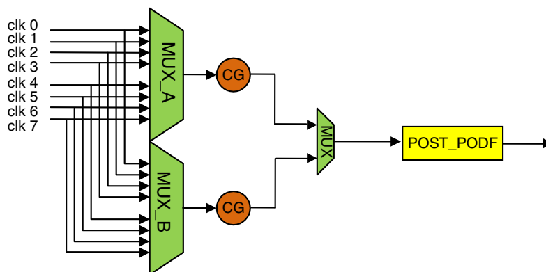
Figure 5-17. Core clock slice
