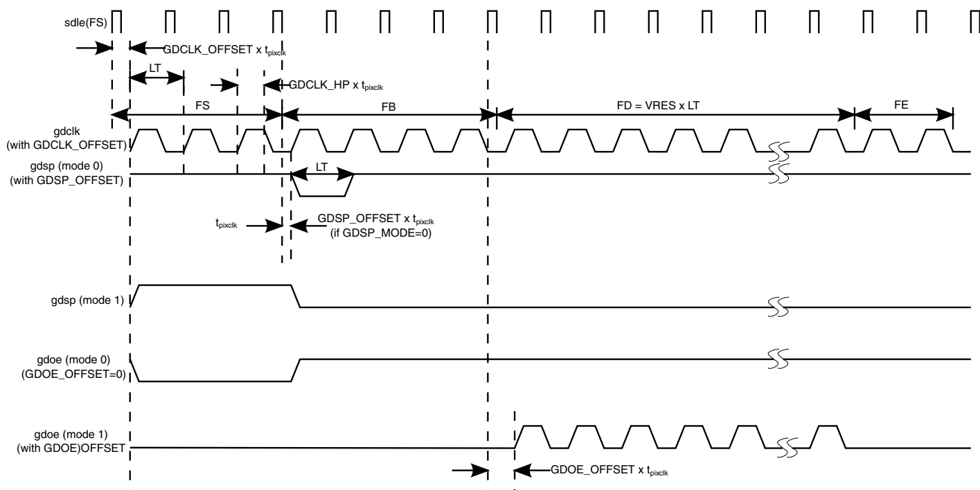
Figure 13-75. Frame Timing (Vertical)
