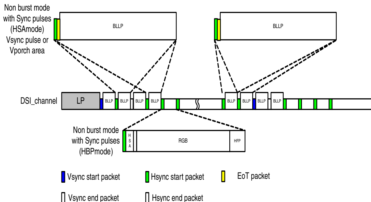
Figure 13-34. Block Timing Diagram of HSE Disable Mode (HSE Mode Reset : \text{DSIM\_CONFIG}[23] = 0 )
