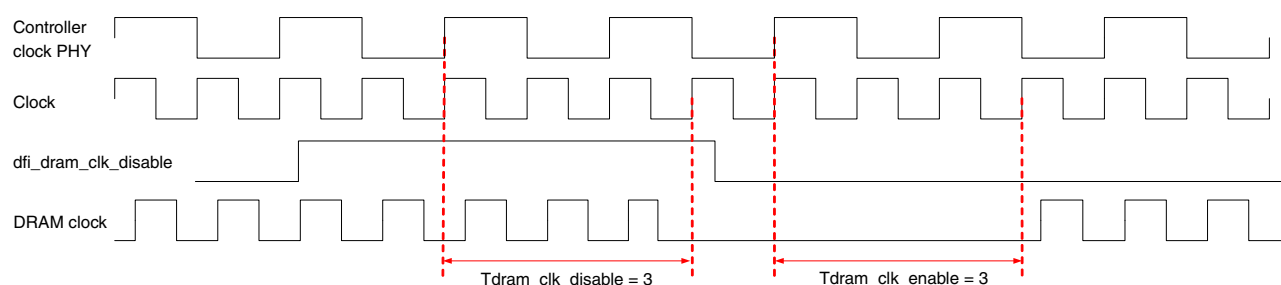
Figure 9-24. Clock Control Timing
