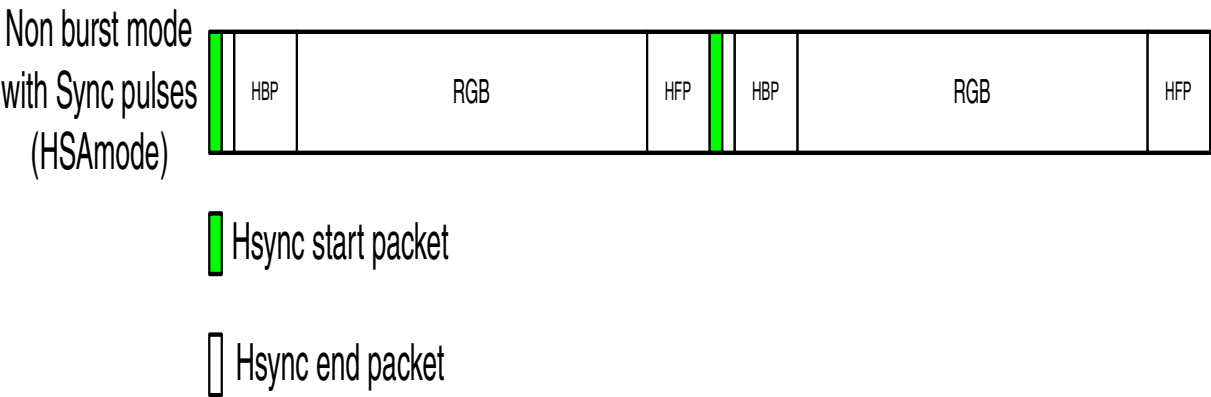
Figure 13-30. Block Timing Diagram of HSA Disable Mode (HSA Mode Reset : DSIM_CONFIG[20] = 1)
