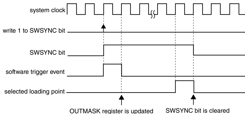
Figure 12-57. OUTMASK synchronization with (SYNCMODE = 0), (SYNCHOM = 1), (PWMSYNC = 0) and software trigger was used
