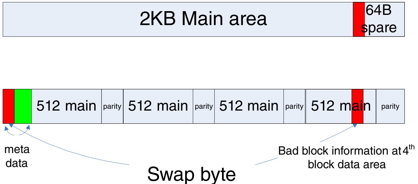
Figure 6-27. Factory Bad Block Marker Preservation
