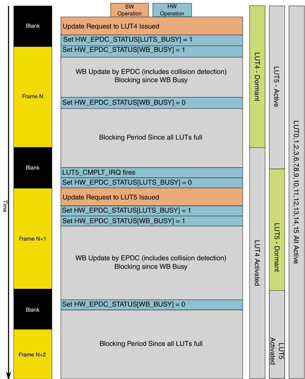
Figure 13-85. Temporal Flow of Update Processing
