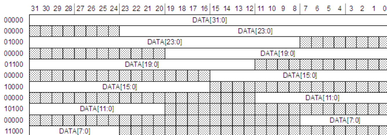
Figure 13-118. SAI first bit shifted, LSB first
