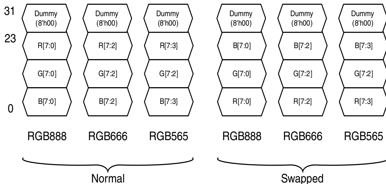
Figure 13-58. RGB Data Alignment
