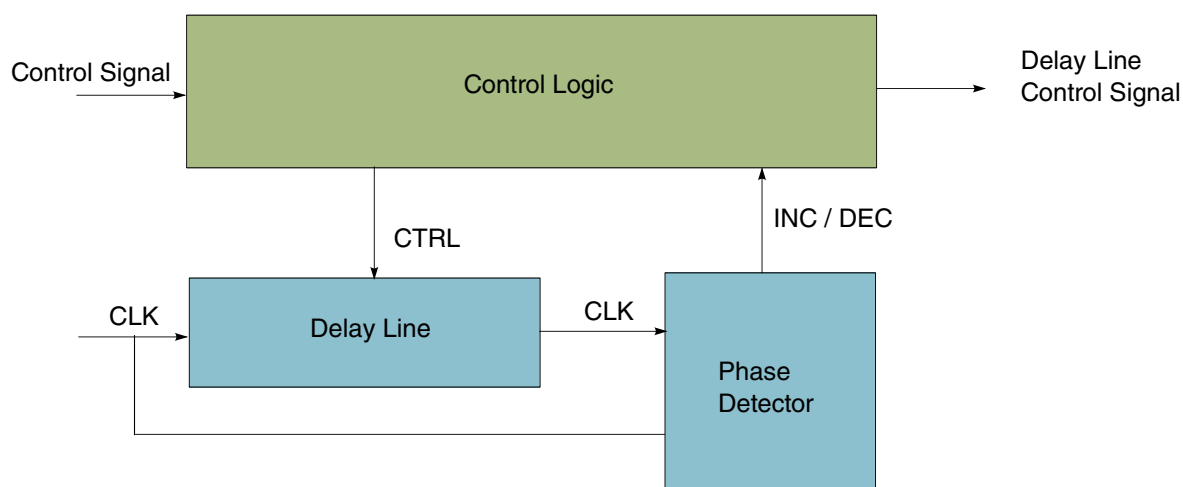
Figure 9-10. Block Diagram of DLL
