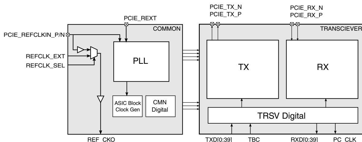
Figure 11-52. Block Diagram
