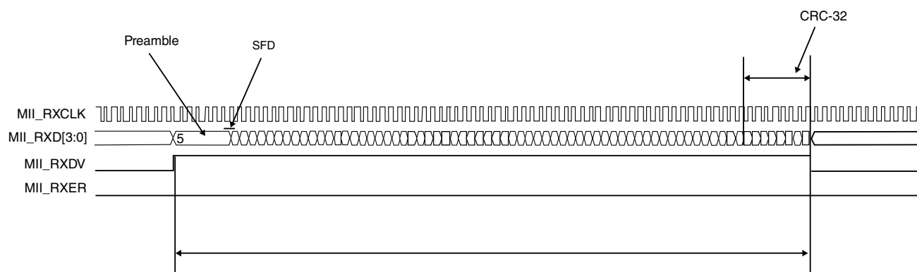
Figure 11-29. MII receive operation
