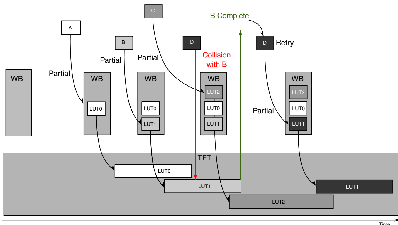
Figure 13-83. Collision Sequence
