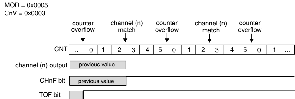
Figure 12-21. Example of the Output Compare mode when the match clears the channel output
