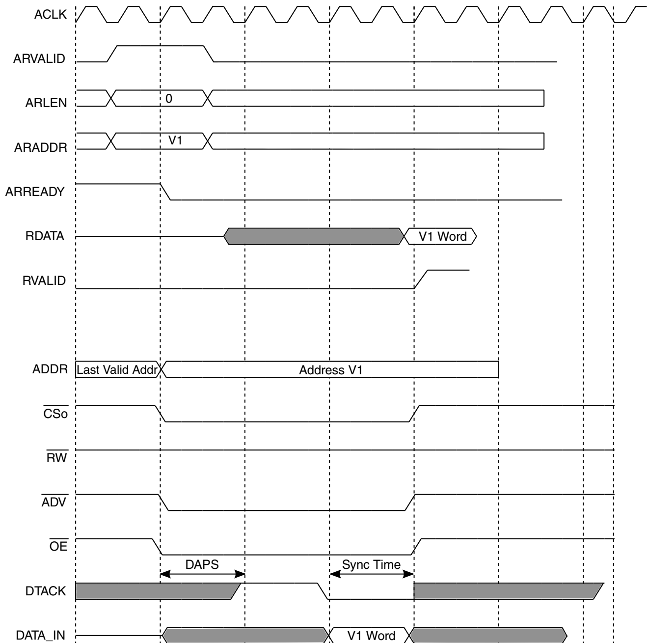
Figure 9-69. DAPS = 2
