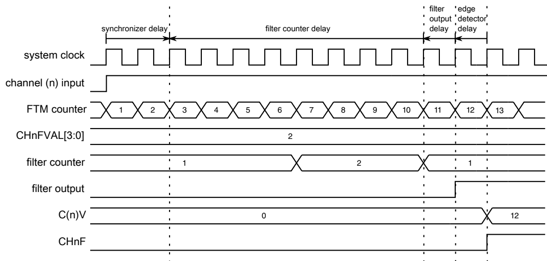
Figure 12-18. Input capture example
