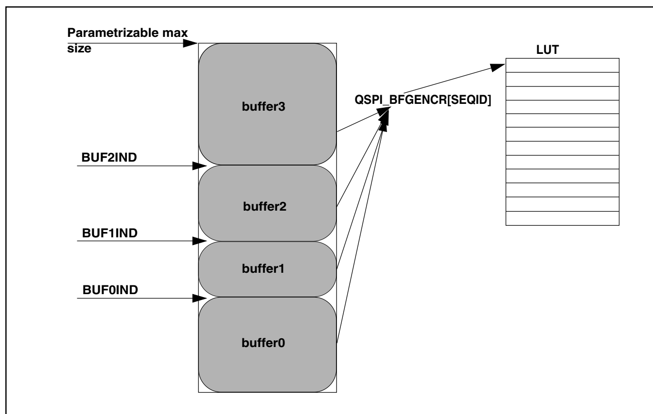
Figure 10-18. Flexible AHB Buffers
