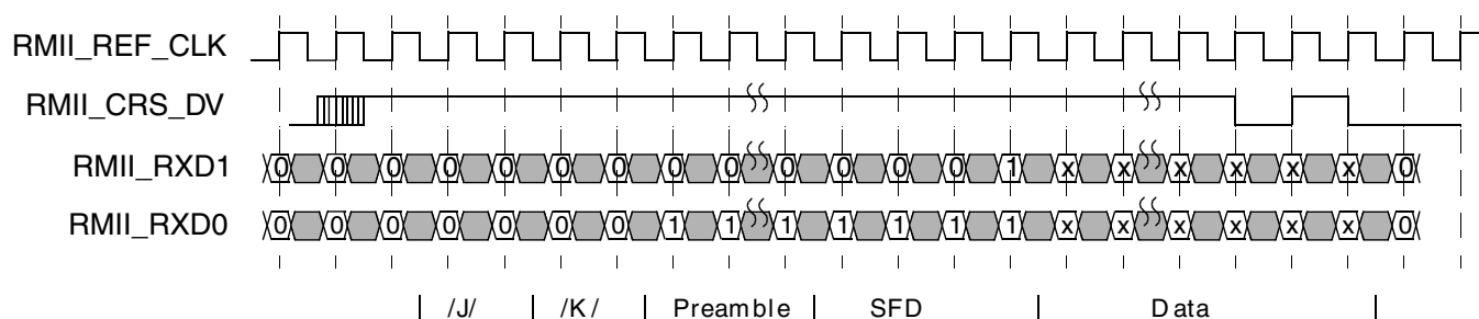
Figure 11-21. RMII receive operation
