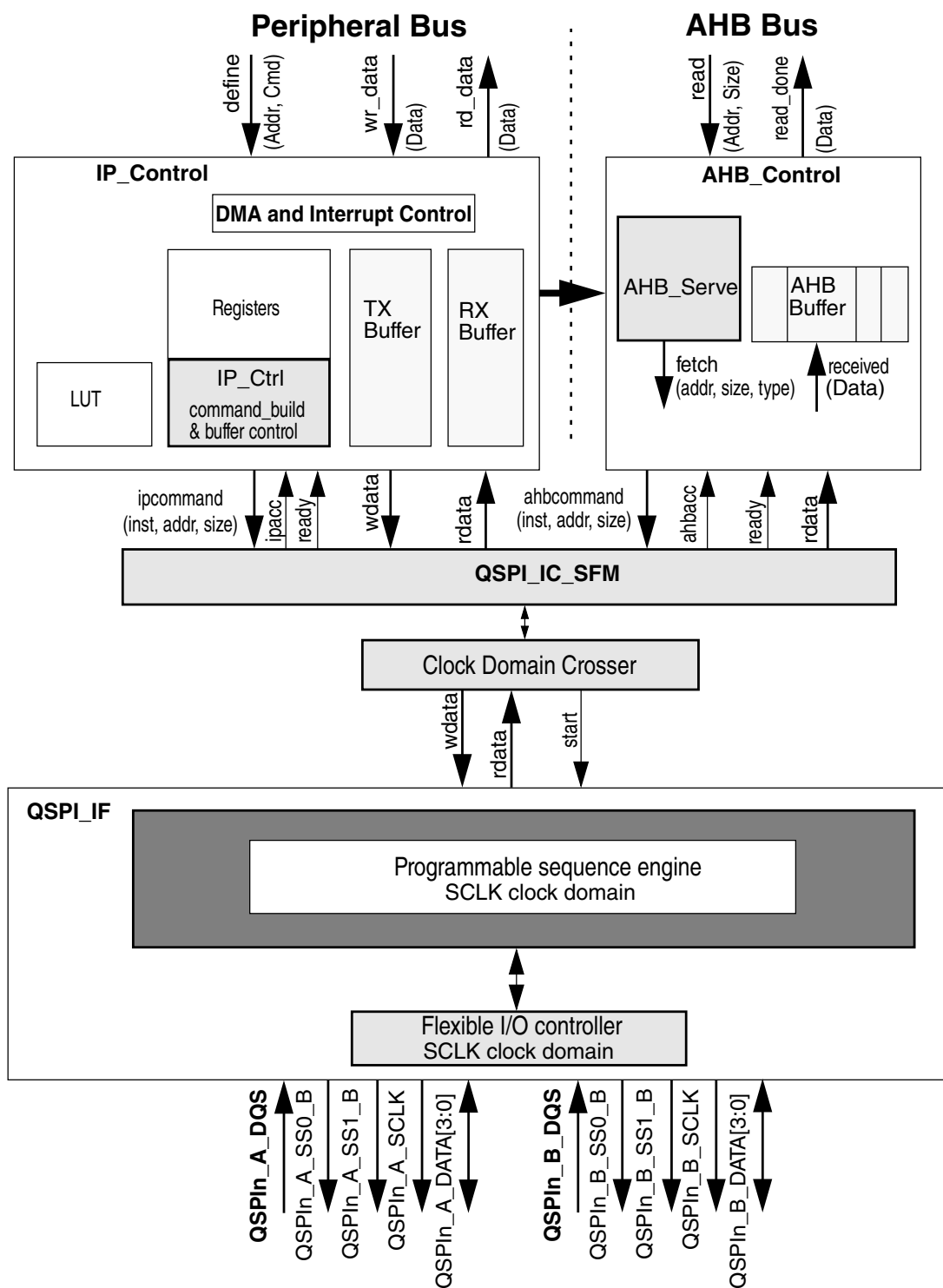
Figure 10-15. QuadSPI Block Diagram
