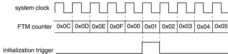
Figure 12-77. Initialization trigger is generated when the FTM counting achieves the CNTIN register value
