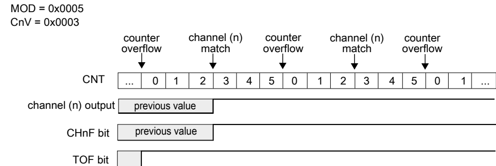
Figure 12-22. Example of the Output Compare mode when the match sets the channel output
