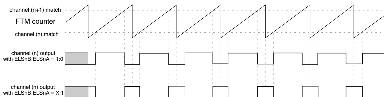
Figure 12-29. Combine mode
