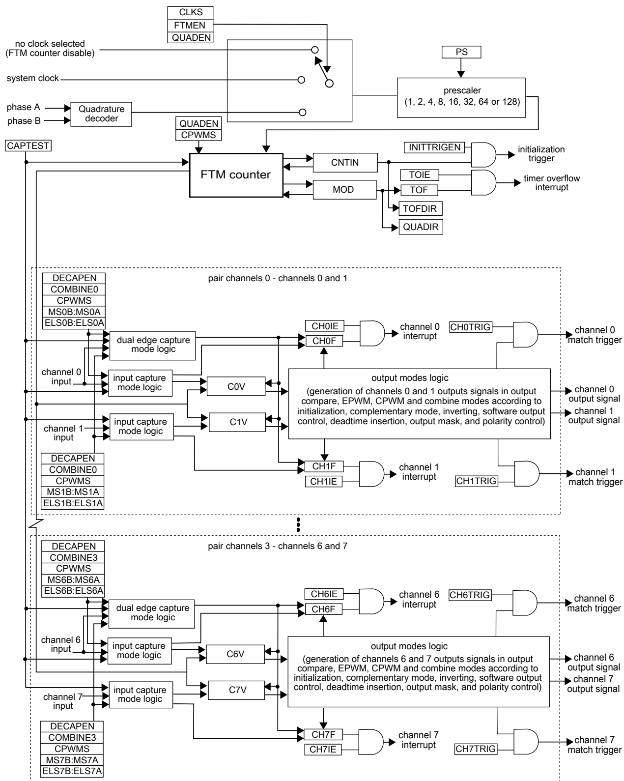
Figure 12-5. FTM block diagram
