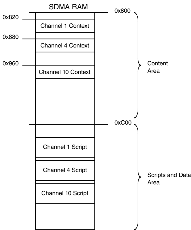
Figure 7-16. Example of SDMA RAM After Boot Session
