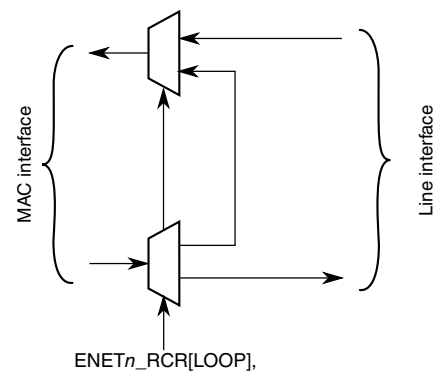
Figure 11-15. Loopback options
