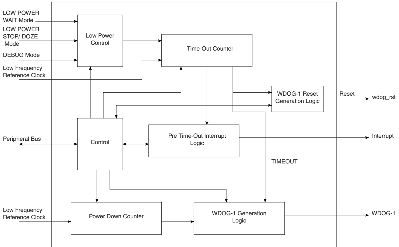
Figure 6-14. WDOG Diagram
