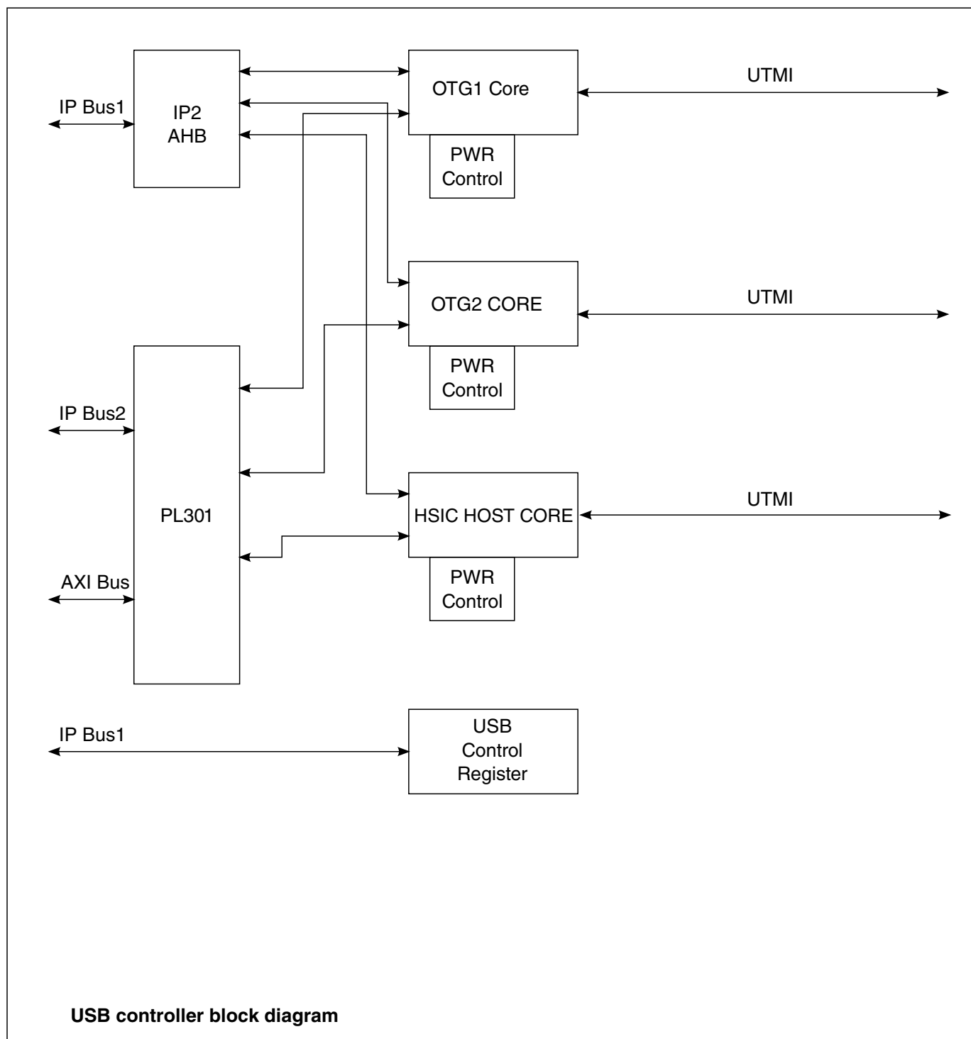
Figure 11-58. USB block diagram
