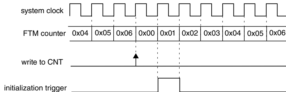
Figure 12-78. Initialization trigger is generated when there is a write to CNT register
