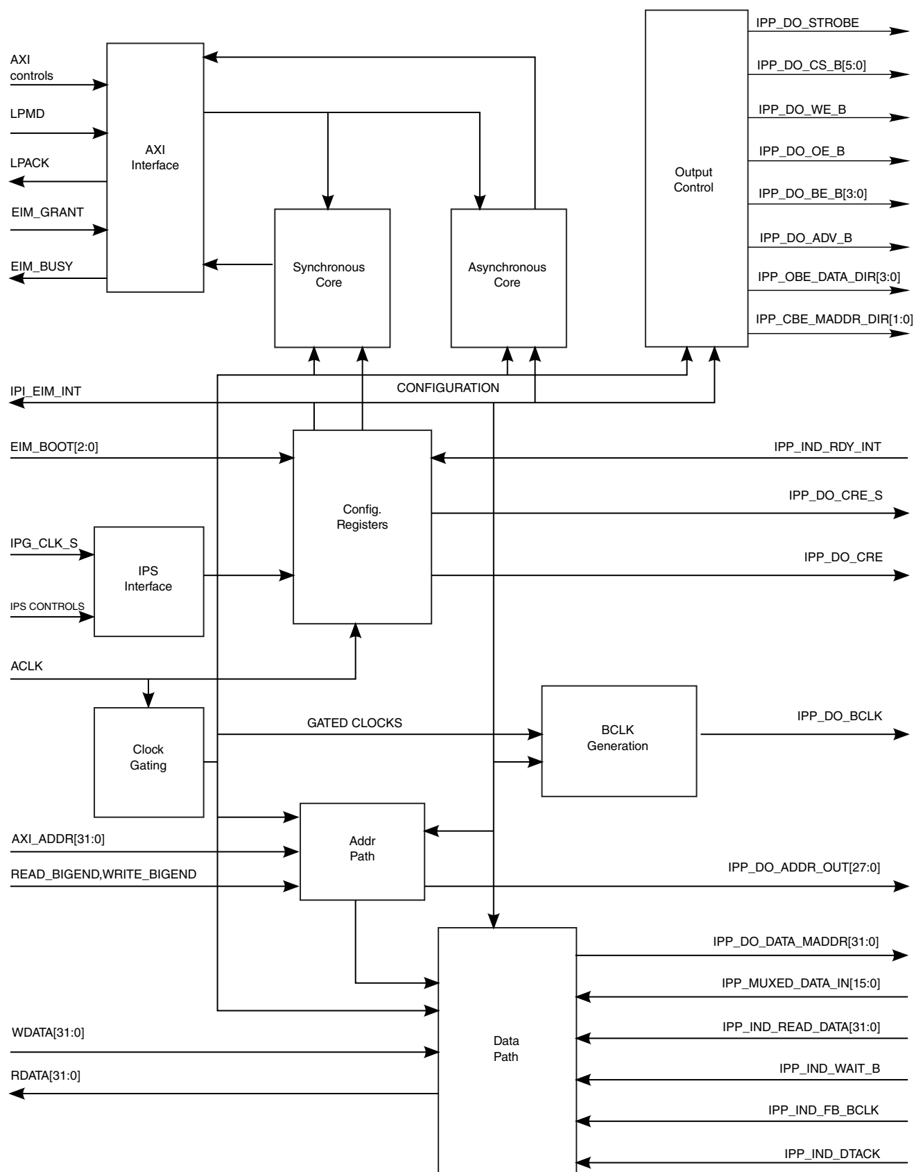
Figure 9-55. EIM Diagram
