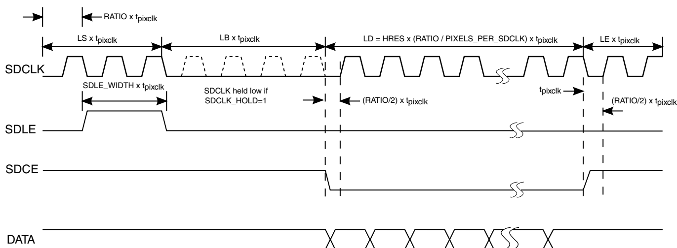
Figure 13-73. Line Timing ( \text{DDR\_MODE} = 0 )
