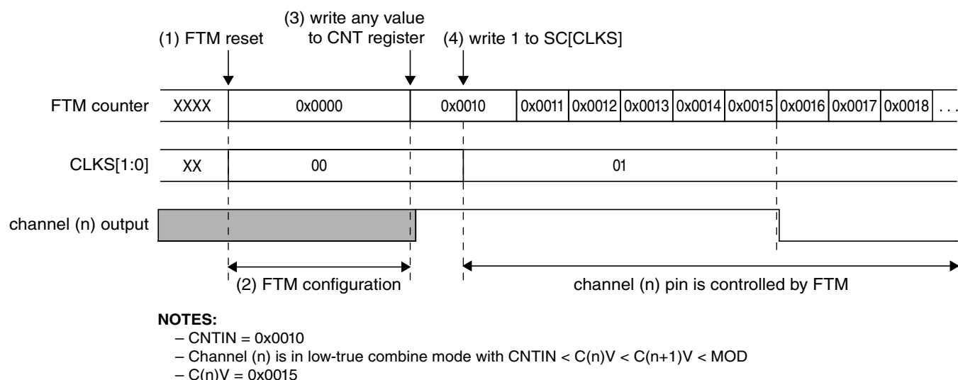
Figure 12-98. FTM behavior after reset when the channel (n) is in Combine mode
