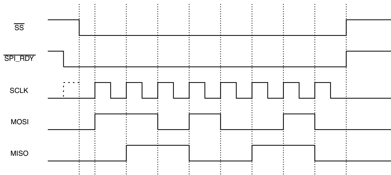
Figure 10-6. Relationship Between a SPI Burst and \overline{\text{SPI\_RDY}} : Low-Level Triggered
