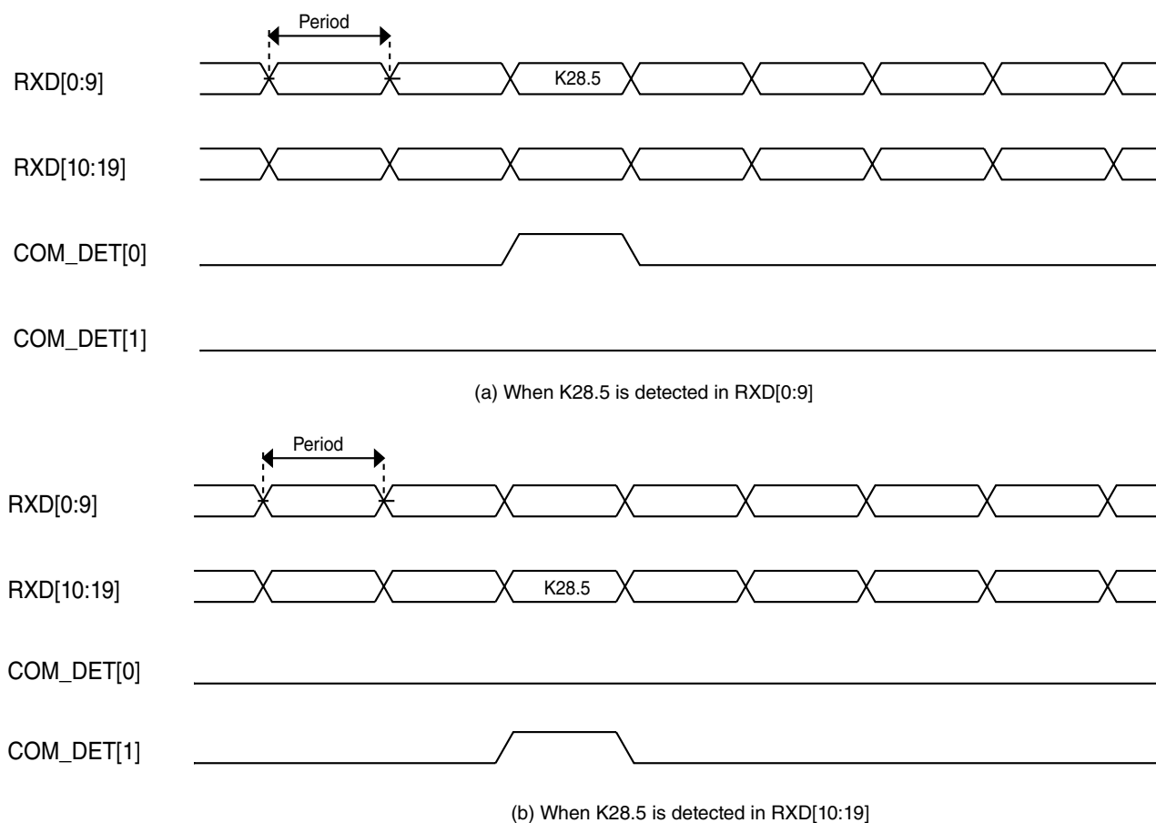
Figure 11-55. Detection of a K28.5 Character
