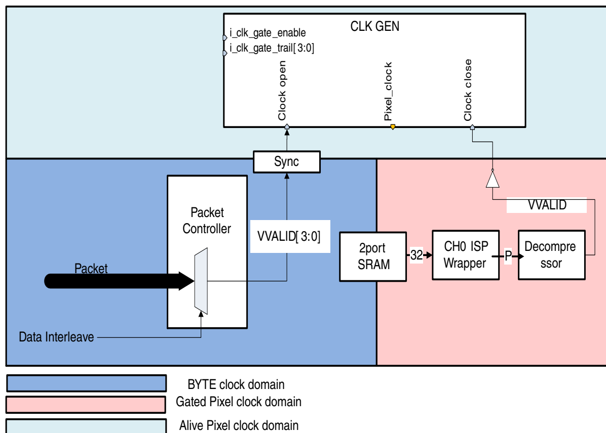
Figure 13-66. Clock Gating Block
