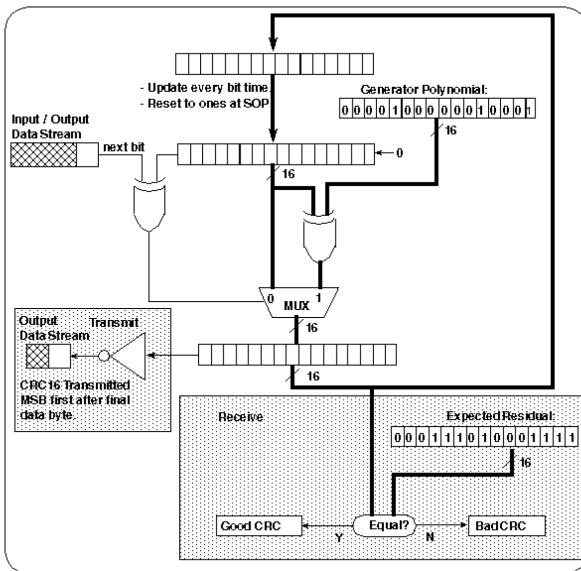
Figure 11-50. CRC Block Diagram
