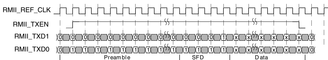
Figure 11-23. RMII transmit operation
