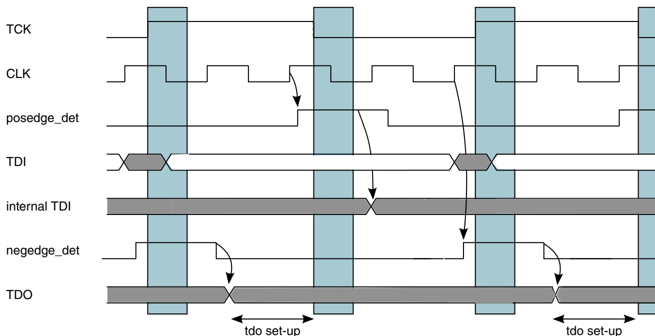
Figure 7-10. Synchronization Timings
