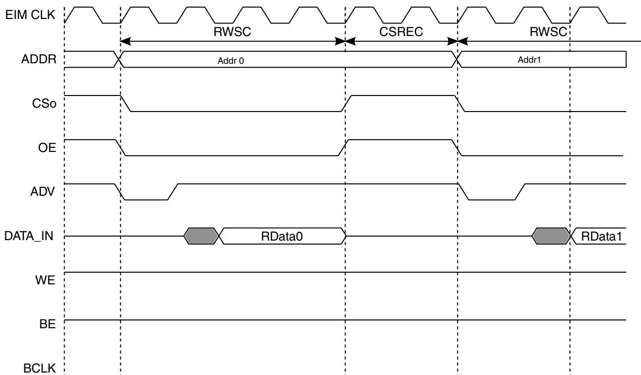
Figure 9-65. RWSC=4, RCSA=0, OEA=0, RADVA=0, RCSN=0, OEN=0, RADVN=0, CSREC=2
