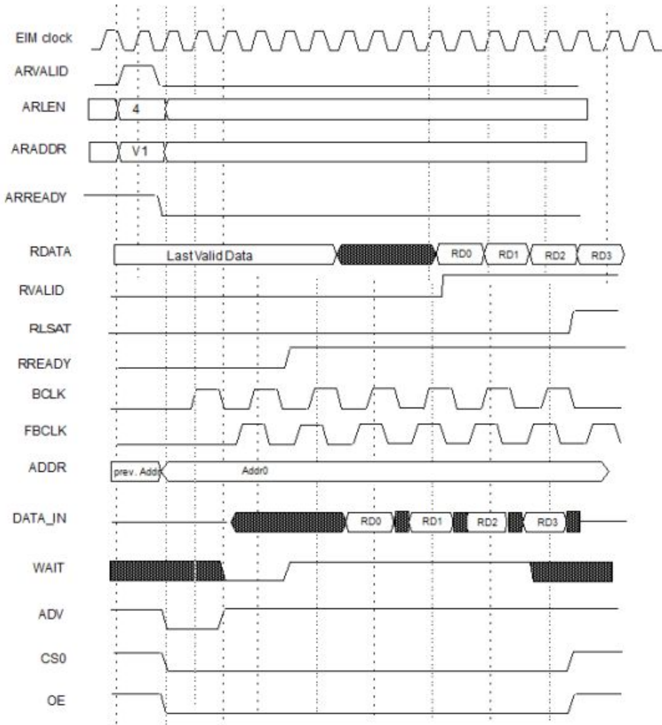
Figure 9-67. BCD=1, RL = 3
