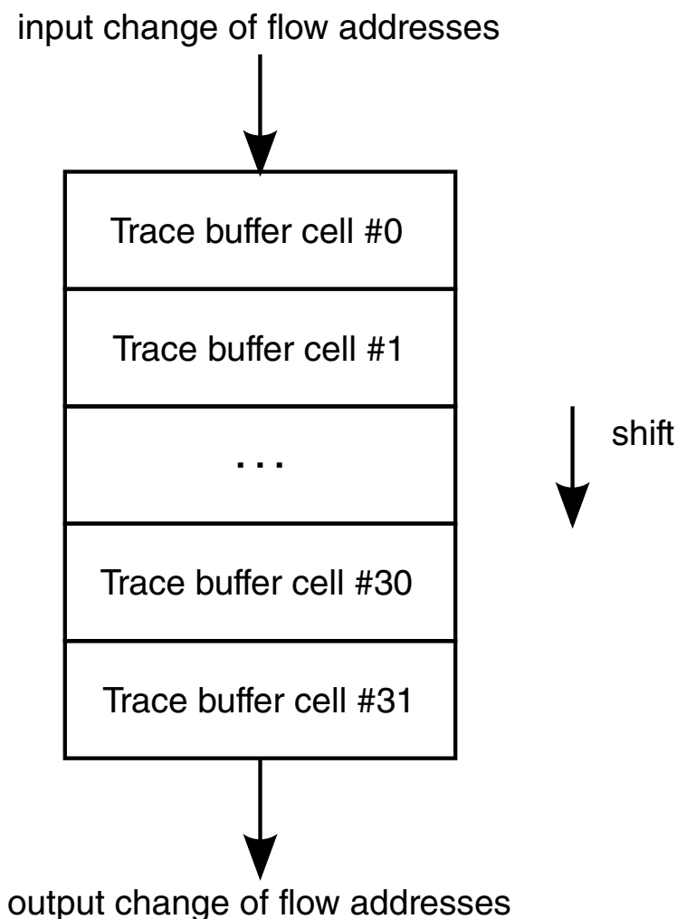
Figure 7-13. Trace Buffer
