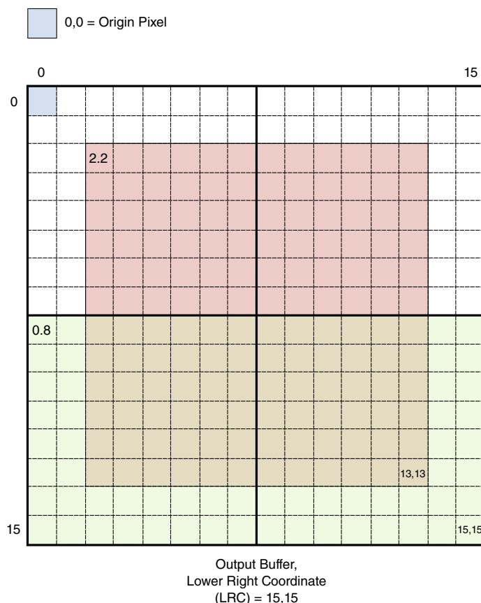
Figure 13-88. Sample output buffer configuration
