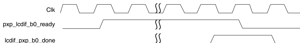
Figure 13-103. Buffer Sharing Protocol
