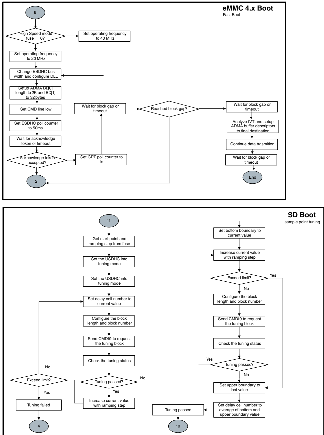
Figure 6-37. Expansion Device Boot Flow (6 of 6) i.MX 7Dual Applications Processor Reference Manual, Rev. 0.1, 08/2016
